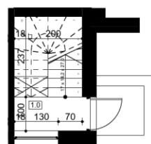
PARTER
